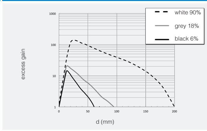
FAI4, FAI5/**-(2,3)* excess gain
